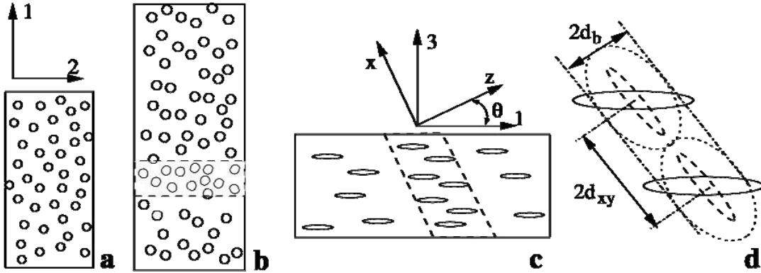
FIGURE 3. LA necking model: Spherical voids with an initial homogeneous distribution (a), in plane virtual localization band after a plastic deformation with vertical major strain (b), through-thickness virtual localization band after a biaxial deformation that rendered the voids oblate (c), method for determining the increased porosity in a virtual localization band (d).
