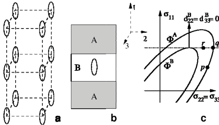
FIGURE 2. Typical coalescence model based on limit analysis: distribution of voids after some deformation (a), elementary cell showing sound and highly porous layers (b) and limit load interpretation of the onset of coalescence with stress states in the sound regions before coalescence p , at the onset of coalescence q and during coalescence r (c).
